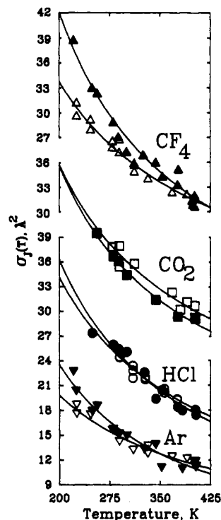
Figure 3. Cross sections for rotational angular momentum transfer \sigma_j for the CH 4 molecule with various collision partners, obtained independently from 13 C (filled symbols) and from 1 H (open symbols) T 1 in CH 4 -CF 4 , CH 4 -CO 2 , CH 4 -HCl, and CH 4 -Ar gas mixtures containing 13 CH 4 and 12 CH 4 , respectively. The curves are the least-squares fit to a power law, \sigma_j(T) = \sigma_j(300 \text{ K})(T/300)^m , where \sigma_j(300 \text{ K}) and m are the values shown in Table IV.
