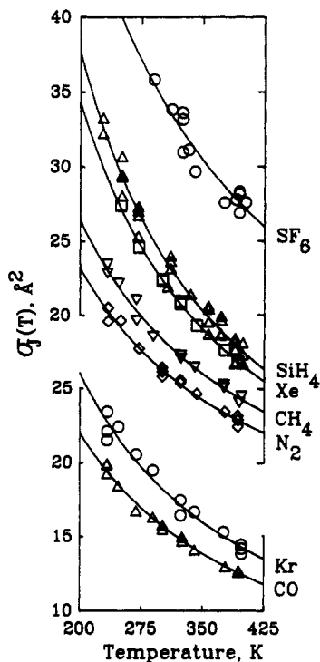
Figure 4. Cross sections for rotational angular momentum transfer \sigma_j for CH 4 molecule in CH 4 -X collisions, obtained from 1 H T 1 in 12 CH 4 molecule in various gases. The curves are the least-squares fit to a power law \sigma_j(T) = \sigma_j(300 \text{ K})(T/300)^m , where \sigma_j(300 \text{ K}) and m are the values shown in Table IV.
