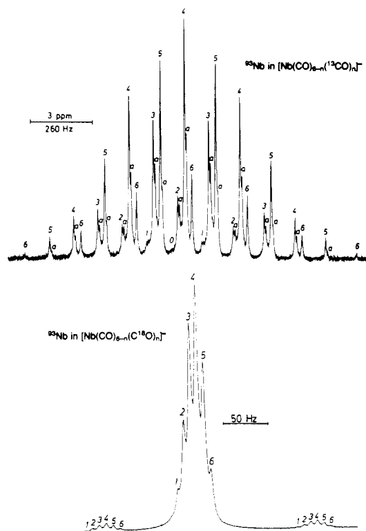
Figure 3. ^{93}\text{Nb} NMR spectra of [\text{Nb}(\text{CO})_6]^- ion (a) enriched in ^{13}\text{C} and (b) enriched in \text{C}^{18}\text{O} taken at 88.29 MHz in acetone solution. Assignments refer to the isotopomers [\text{Nb}(^{12}\text{C}^{16}\text{O})_{6-n}(^{13}\text{CO})_n]^- and [\text{Nb}(^{12}\text{C}^{16}\text{O})_{6-n}(\text{C}^{18}\text{O})_n]^- respectively, for n = 0-6 . The central group of signals in part b is flanked by the natural-abundance ^{13}\text{C} satellite doublets; ^1J(^{13}\text{C}-^{93}\text{Nb}) = 236 Hz. The peaks marked a in part a are discussed in the text.
